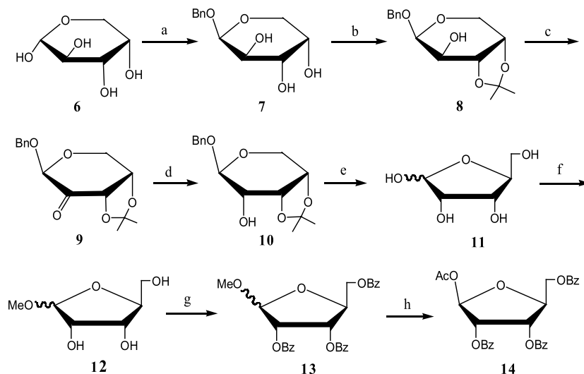
Scheme 2. Synthesis of 1- O -acetyl-2,3,5-tri- O -benzoyl-β- L -ribofuranose. Reagents and conditions: (a) HCl (g)/BnOH; (b) DMP, acetone; (c) PDC, Ac 2 O, CH 2 Cl 2 , reflux; (d) NaBH 4 , MeOH; (e) 4% CF 3 COOH, reflux; (f) 1% HCl (g)/MeOH; (g) BzCl, pyridine; (h) AcOH, Ac 2 O, concd H 2 SO 4 .
