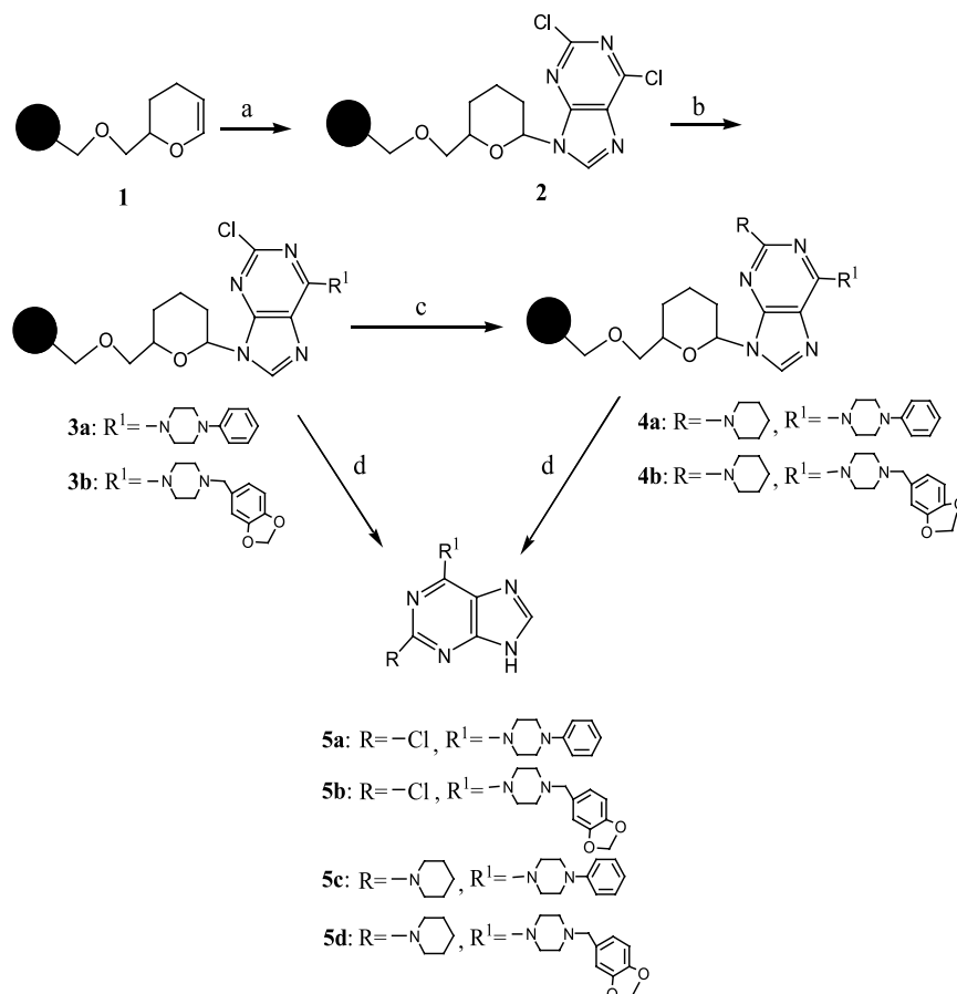
Scheme 1. Solid-phase synthesis of purine analogs. Reagents and conditions: (a) 2,6-dichloropurine, CSA, CH_2Cl_2 , 60 °C; (b) 1-phenyl piperazine or 1-piperonylpiperazine, n -BuOH, Et_3N , 80 °C; (c) piperidine, 102 °C; (d) TFA/ CH_2Cl_2 .
