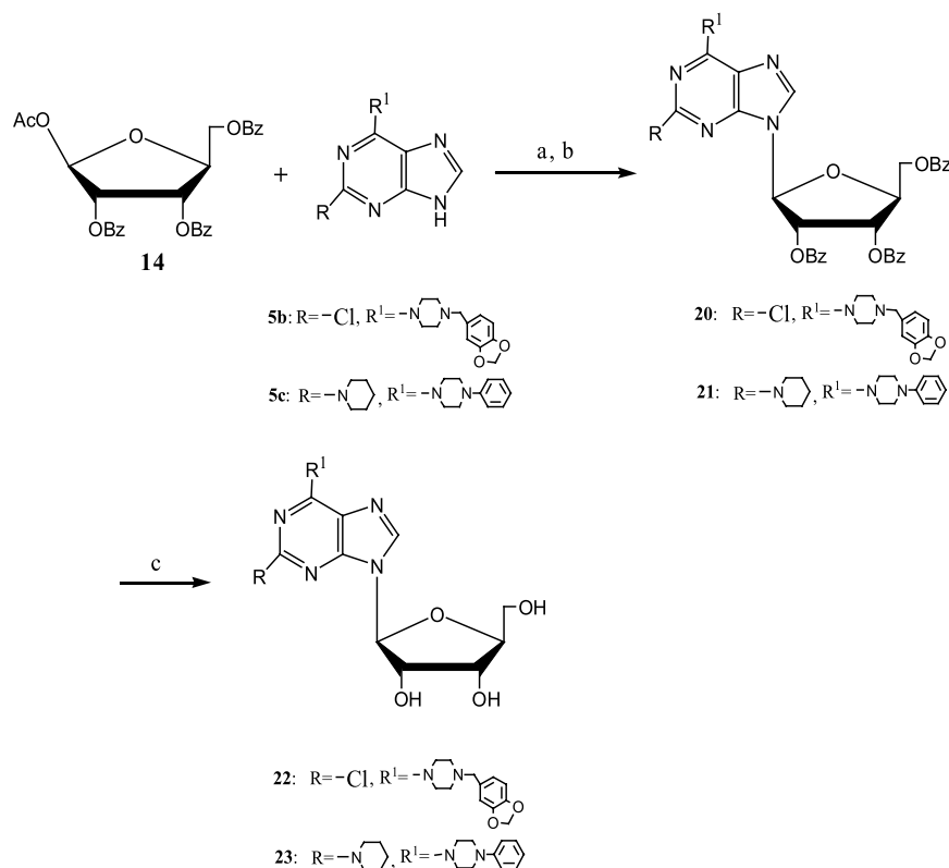
Scheme 4. Synthesis of novel L-purine nucleoside analogs. Reagents and conditions: (a) HMDS, (NH 4 )SO 4 , reflux; (b) TMSOTf, DCE, rt; (c) NH 3 /CH 3 OH.
