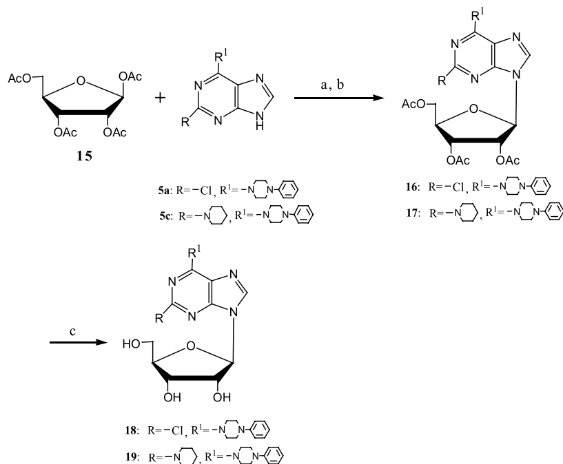
Scheme 3. Synthesis of novel D-purine nucleoside analogs. Reagents and conditions: (a) HMDS, (NH 4 )SO 4 , reflux; (b) TMSOTf, DCE, rt; (c) NH 3 /CH 3 OH.
